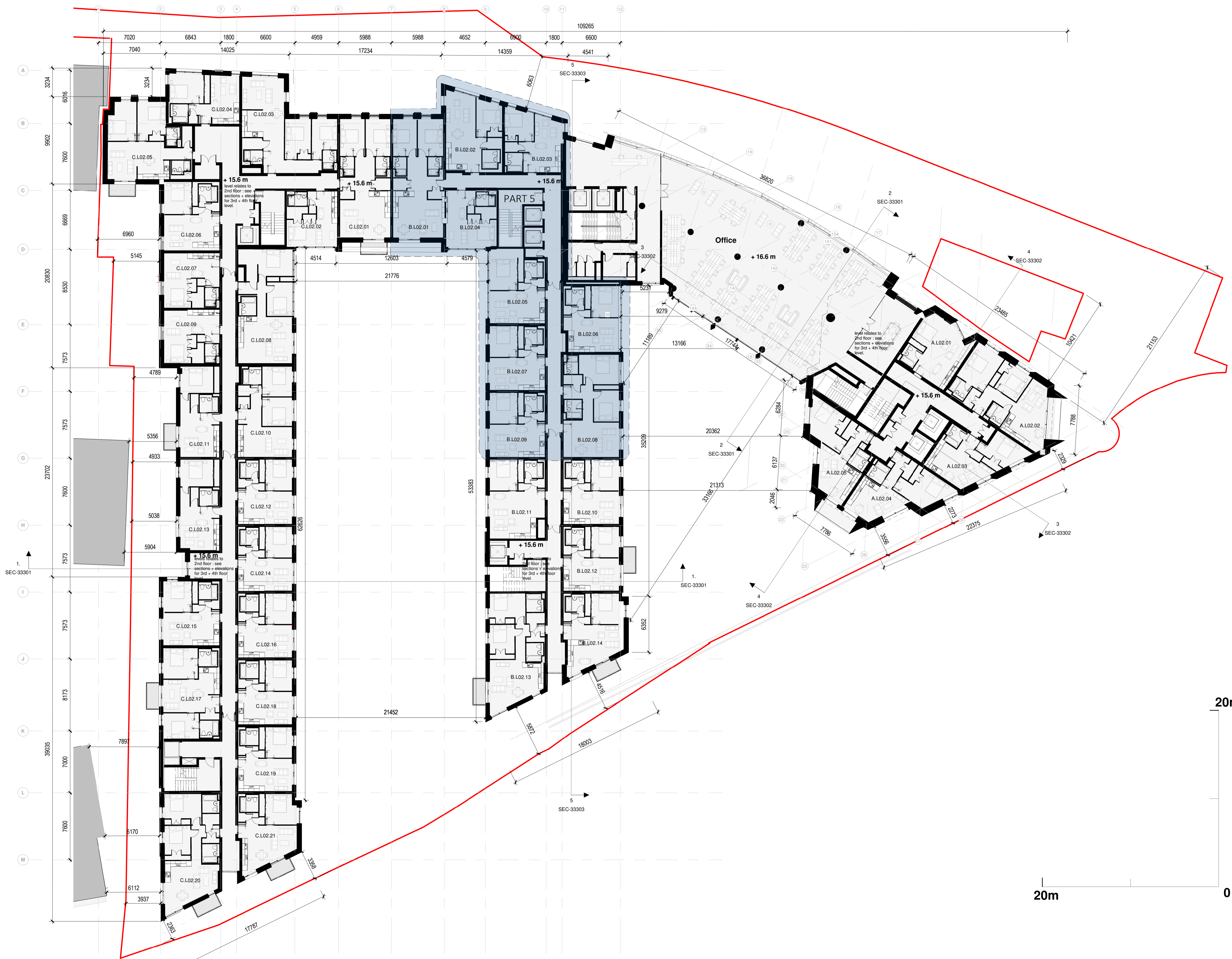
Proposed 2nd - 4th Floor Plan 1 : 200
